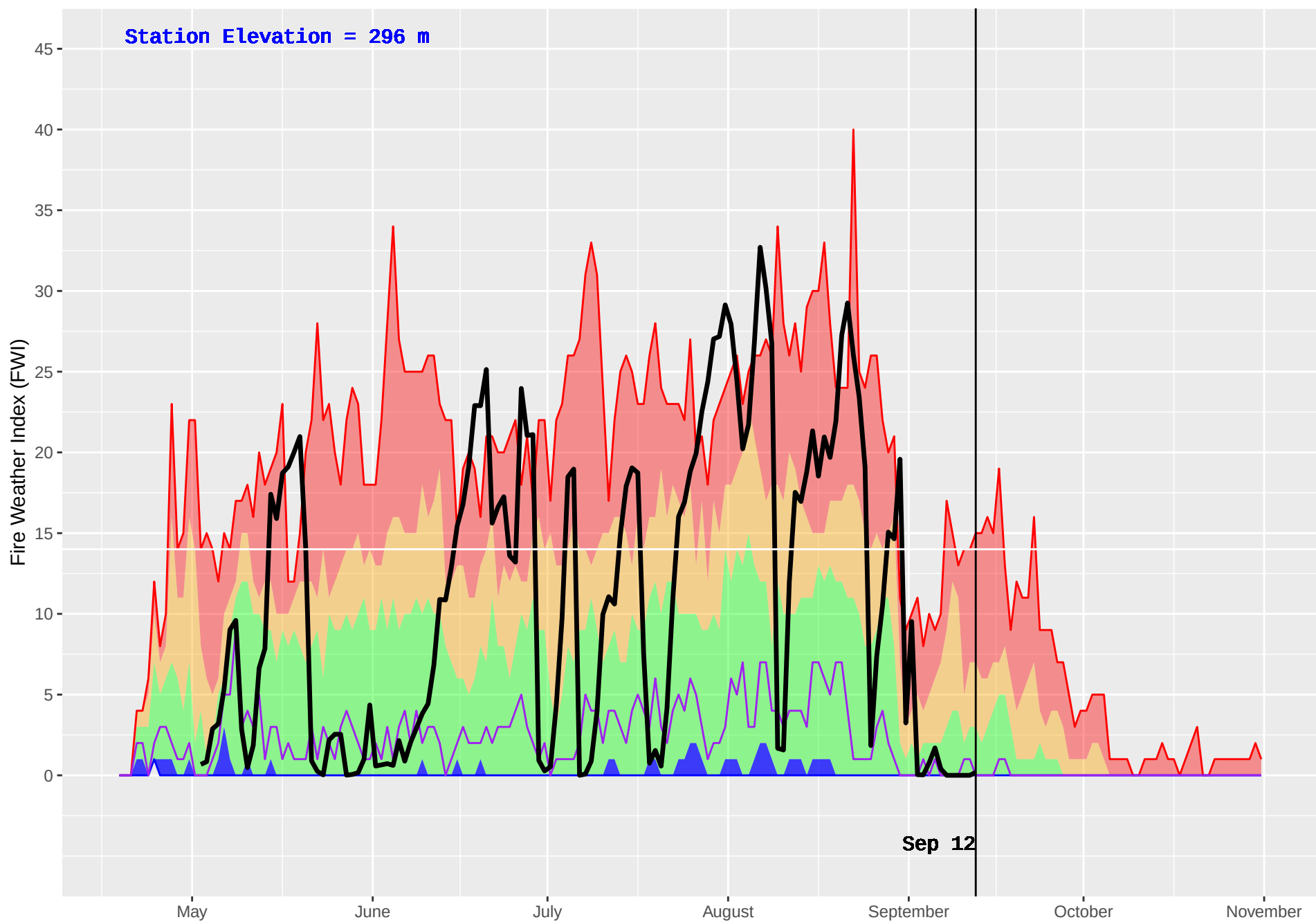
VAN DYKE (430) : Historical (1983–2016) and Current (2018) Daily Fire Weather Index (FWI)
